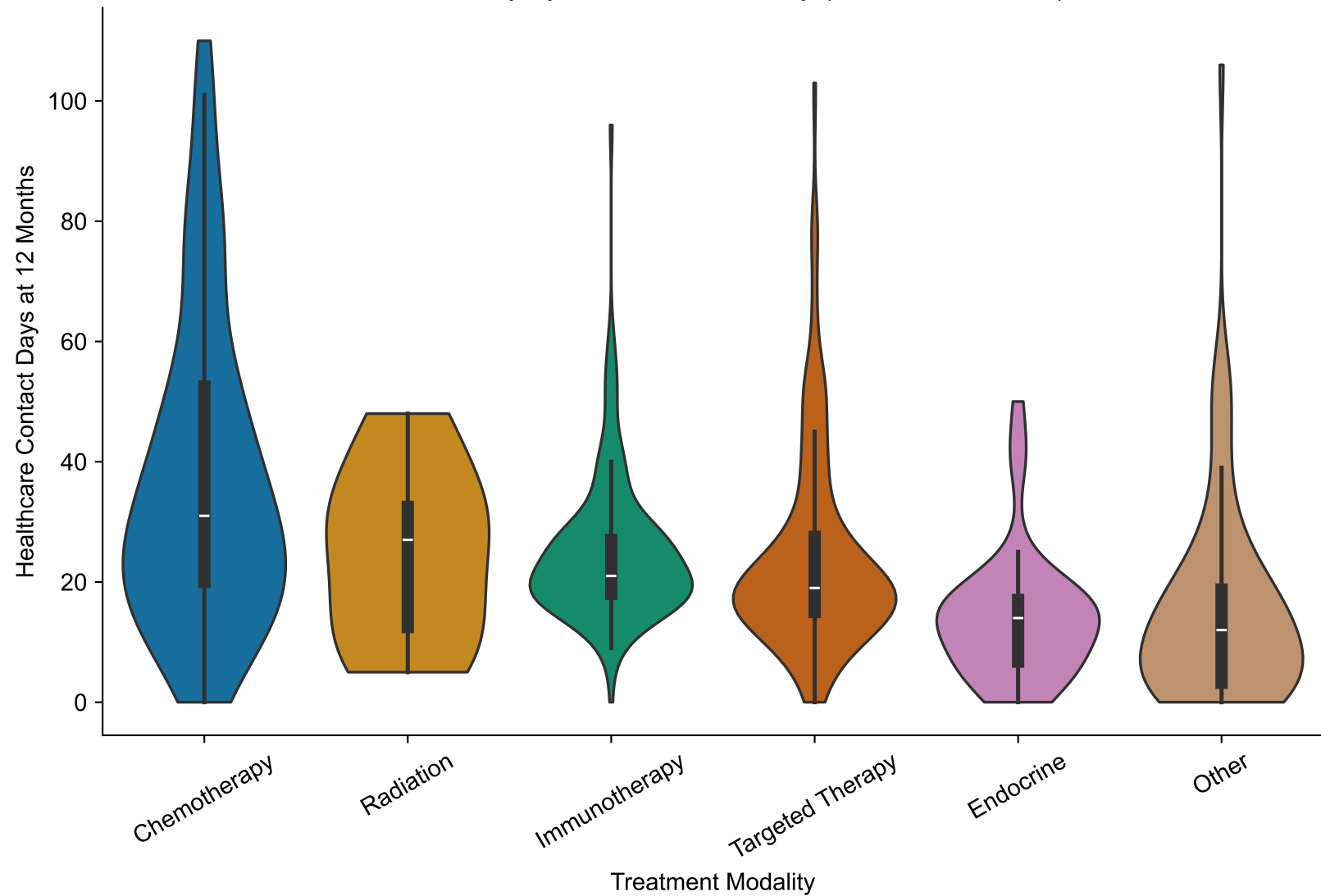
Time Toxicity by Treatment Modality (Intervention Arms)
